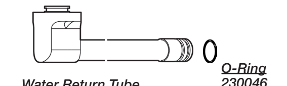
Water Return Tube 450869 4" 450870 6" 450871 8"
