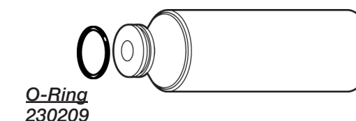
Combustion Chamber 450924
