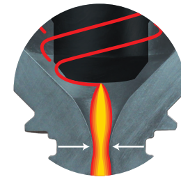
Choked Flow Pressurizes Plasma Arc
